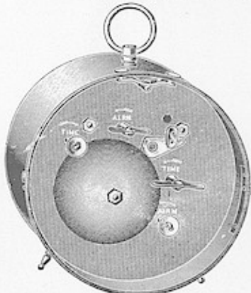
This Cut Represents the General Appearance of New Back and Keys of Parker Rotary Alarm.
