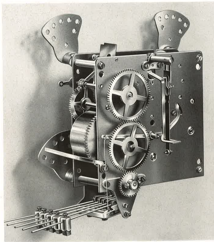
Platinen Plates Platines Platinas 11×11,2 cm
