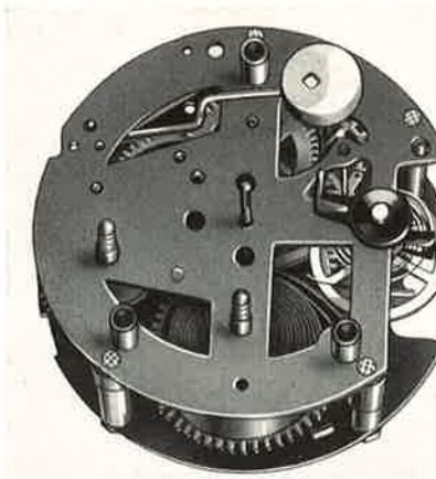
No. 21 1-TAG-MIDGET-WECKERWERK 30-HOUR MIDGET ALARM MOVEMENT MOUVEMENT-REVEIL 30 HEURES "MIDGET" MAQUINA DESPERTADOR 30 HORAS "MIDGET"
