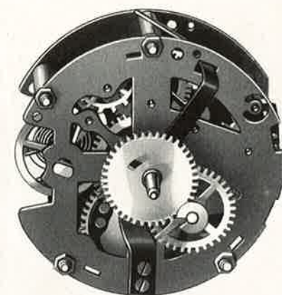
No. 21 1-TAG-MIDGET-WECKERWERK 30-HOUR MIDGET ALARM MOVEMENT MOUVEMENT-REVEIL 30 HEURES "MIDGET" MAQUINA DESPERTADOR 30 HORAS "MIDGET"
