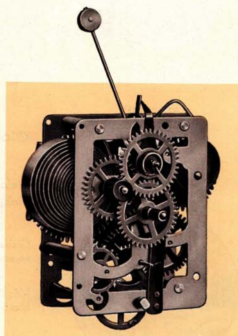
Platinengröße — Size of plates — Medidas de las platinas — Dimensions des platines 76×59 mm = 3×2⅝ inches
