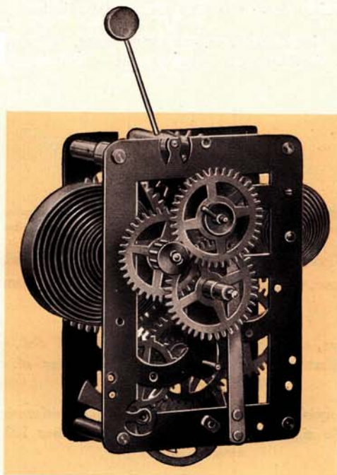
Platinengröße — Size of plates — Medidas de las platinas — Dimensions des platines 83×59 mm = 3¼×2⅝ inches
